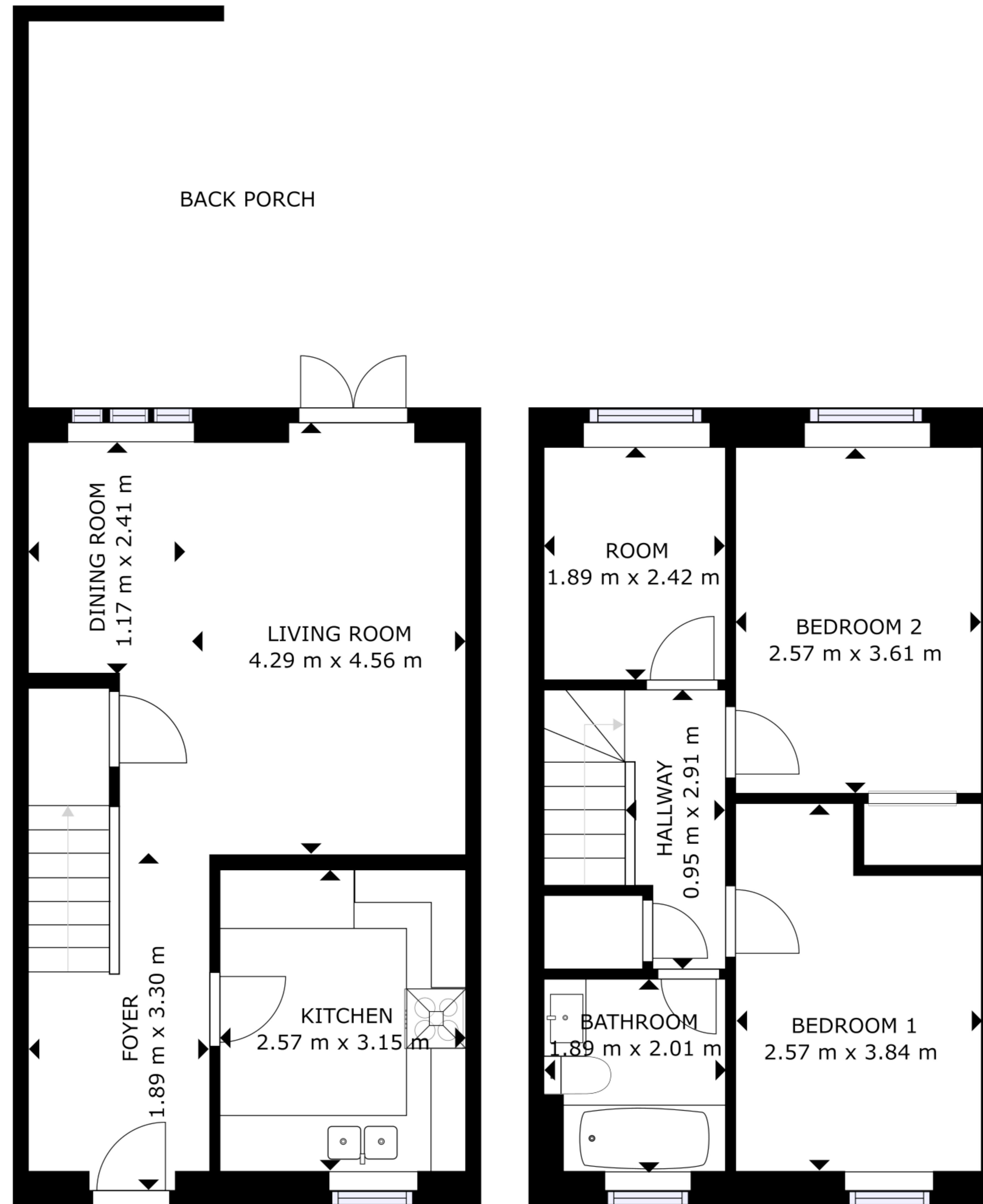
GROUND FLOOR
