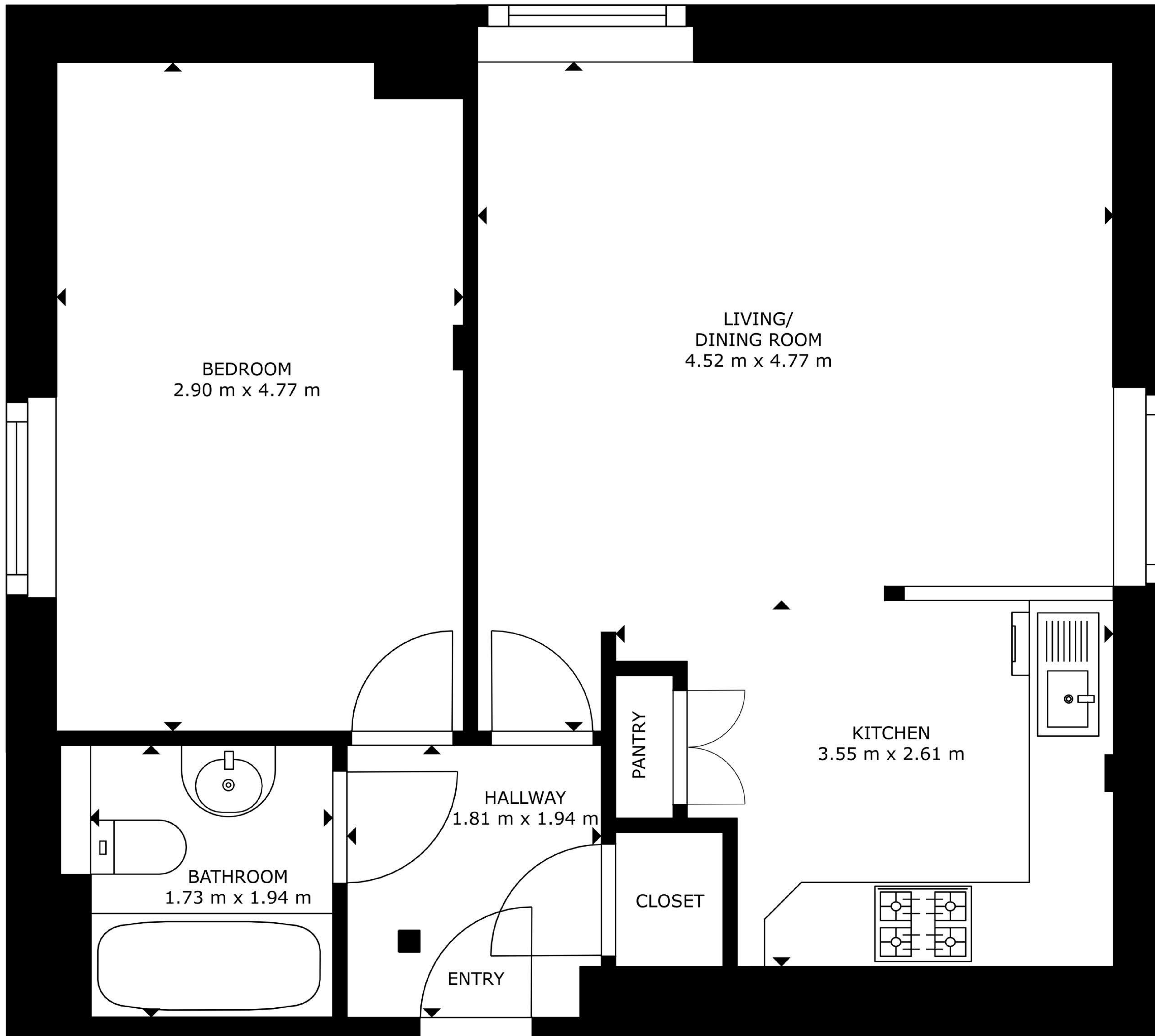
FLOOR PLAN
