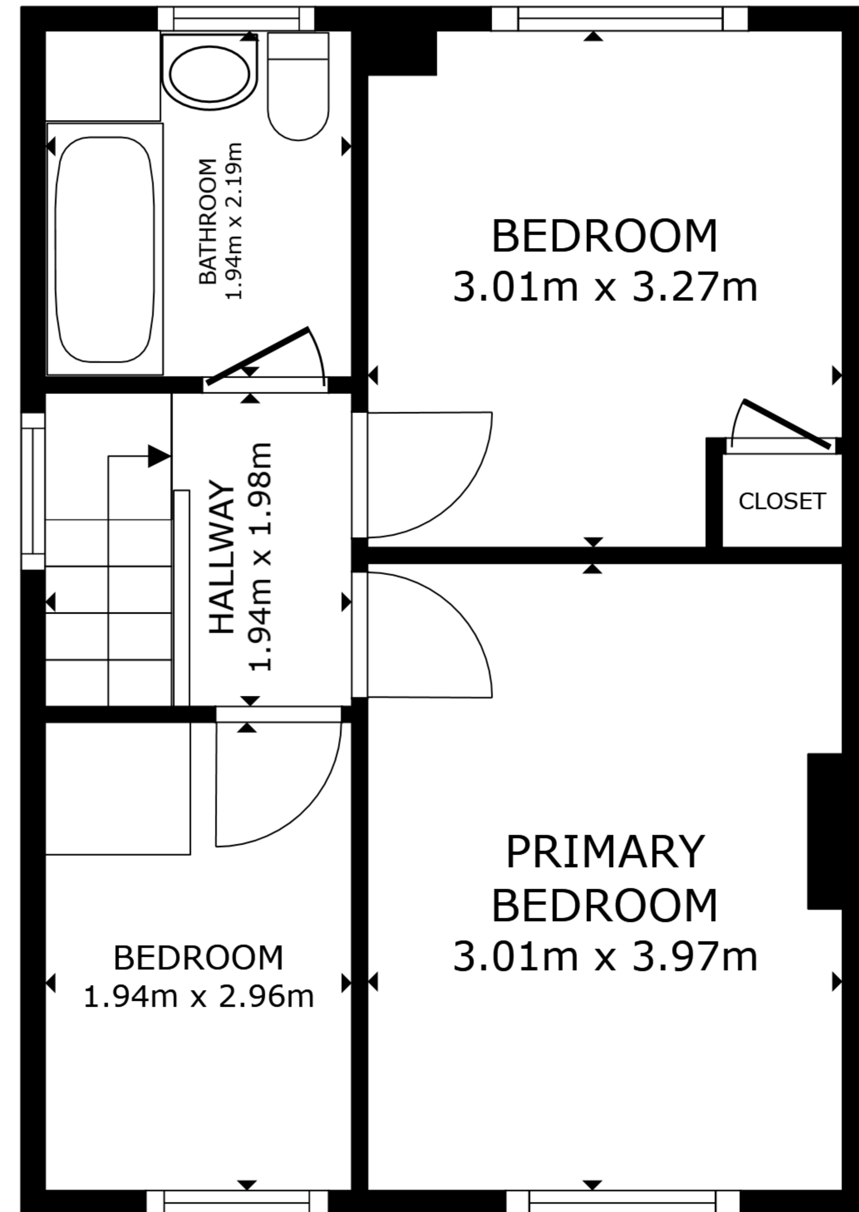
FLOOR 2
